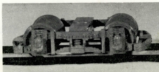
77EXWG Trail Truck with 26" wheels illustrating the new wheel guard for the Eastern Mass 6000- 7000 series cars.
