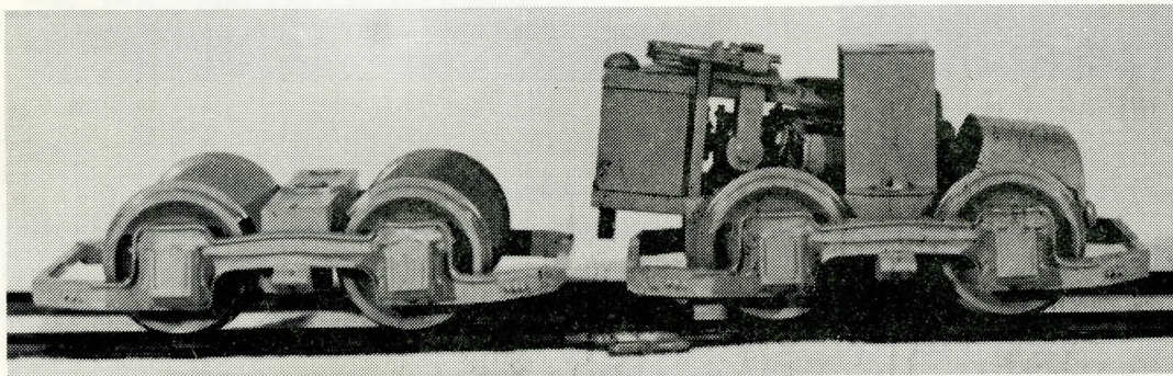
StL47C DC60 Power Truck and Trailer for Chicago 1101-1423 series cars
