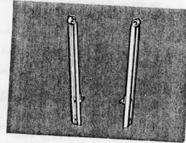
HS-87 HANDRAIL STANCHIONS Fits most G.E. diesels. Beryllium copper, cored for 0.020 handrail wire
