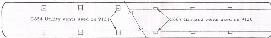
9121 ARCH ROOF
