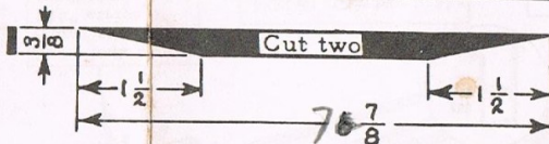
Underframe Assembly Detail
